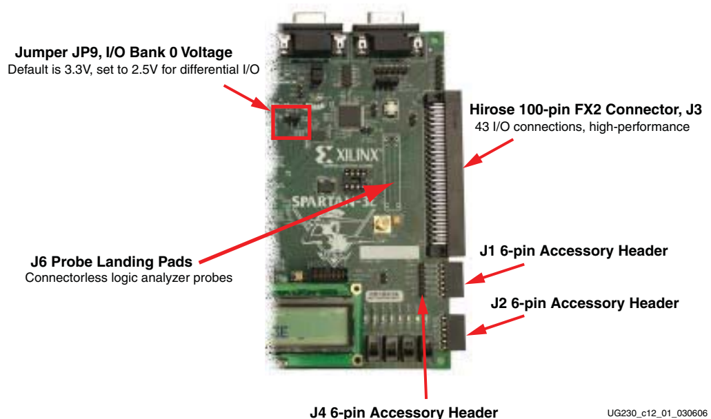
Figure 15-1: Expansion Headers
