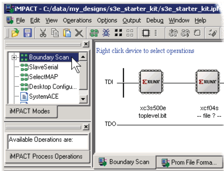
Figure 4-22: Switch to Boundary Scan Mode
